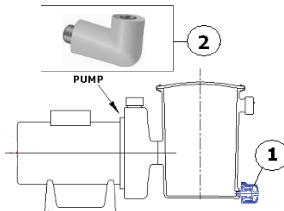
Figure 1. Breather II System Schematic
